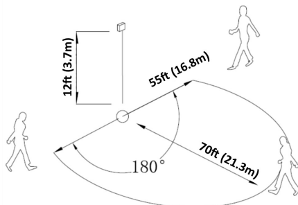
Dipswitches rotated 90°
